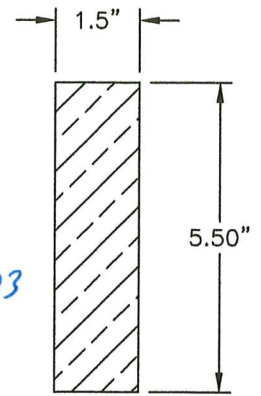
4 1-1/2" X 5-1/2" WOOD CURB SOUTHERN YELLOW PINE 0.55 SG.
