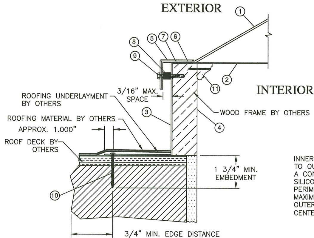
A TYPICAL SECTION - 6" FRAME WOOD SUBSTRATE
